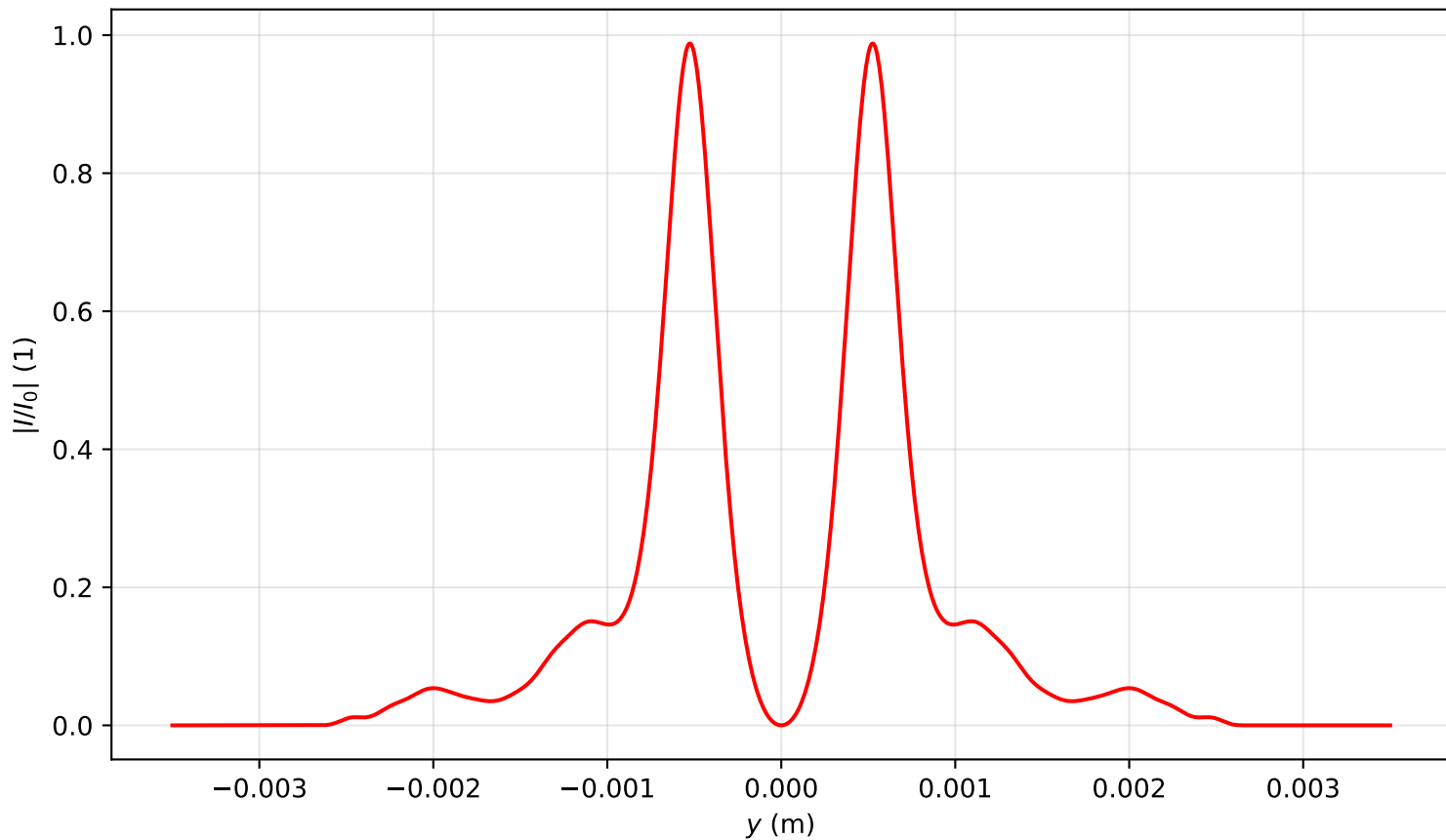
Intensity profile I(x=0, y, z=2.149)/I_0 , \text{Pin}=6.0\text{Pcr} , artificial time
